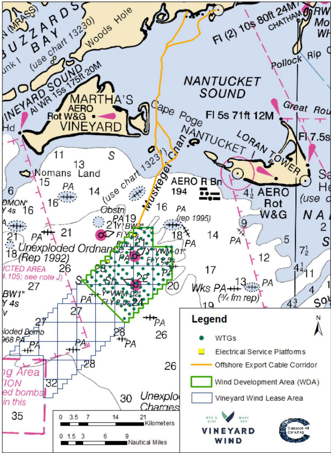
Figure 2.1.3-1 Turbine Layout and Export Cable System
