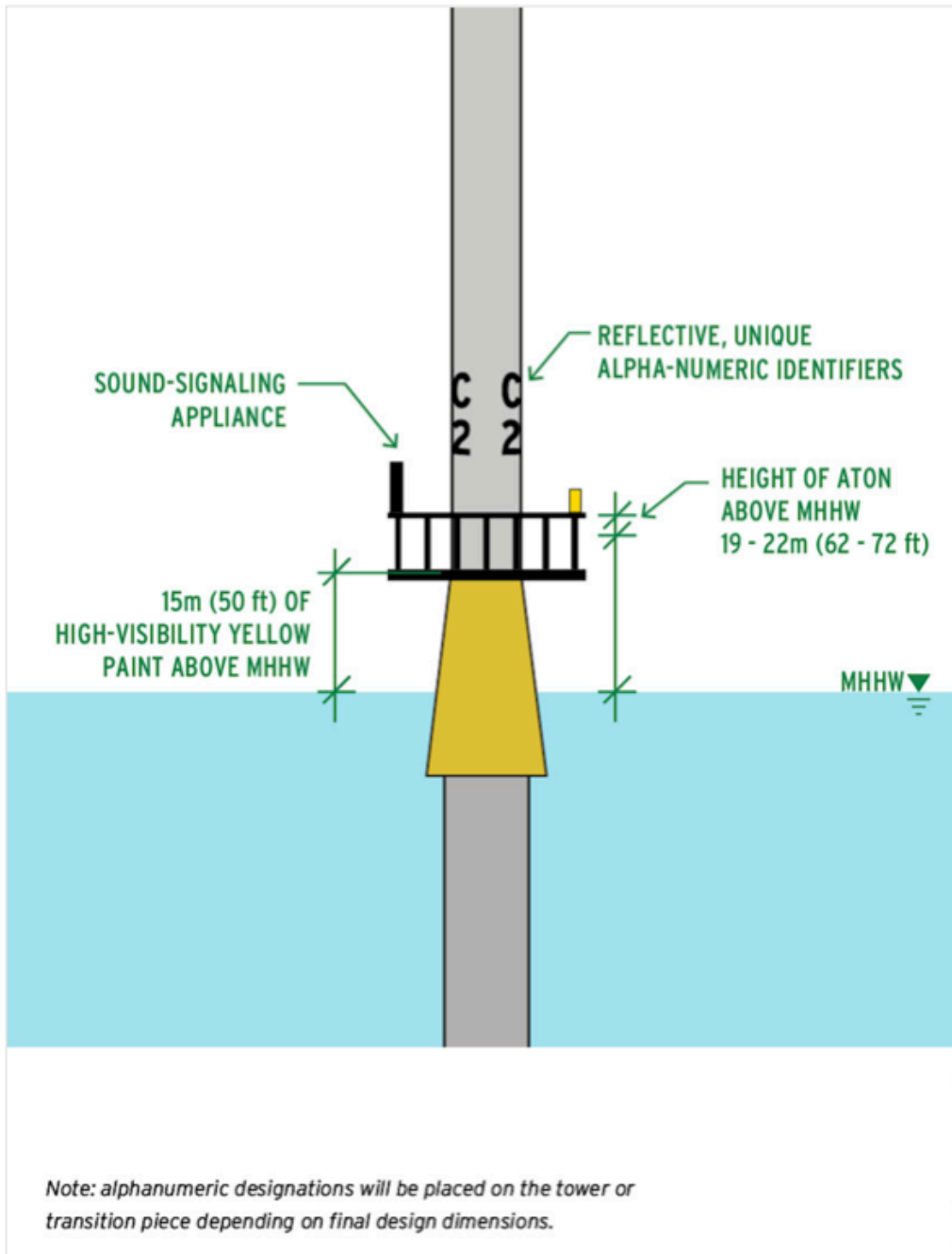
Figure 5.4.2-1 Reflective identifiers and high visibility marking scenario for WTGs in the Project Area.
